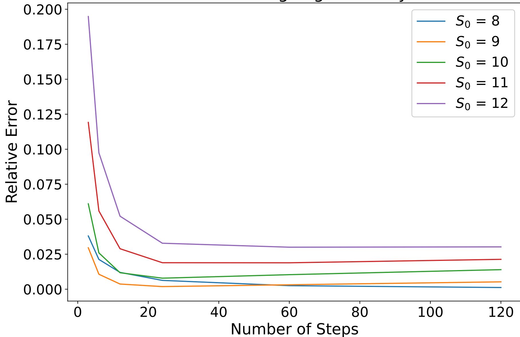
Relative Errors using Laguerre Polynomials
